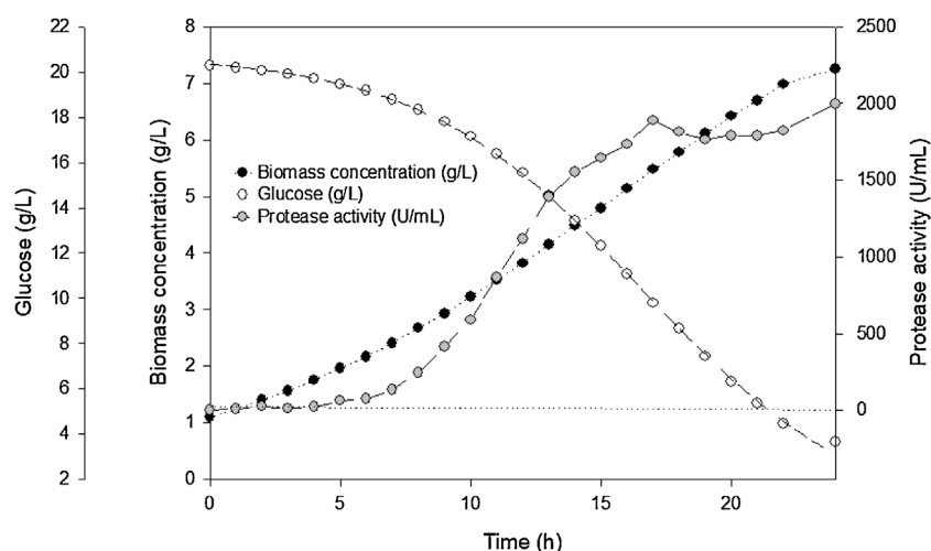
Fig. 5. Time course of a batch culture of R. mucilaginosa CBMAI 1528 in bioreactor. The strain was cultured on medium containing 20 g/L glucose and 10 g/L of casein tryptone for 24 h at 20 °C, pH 5.6, 200 vvm, 500 rpm and K_{La} = 92 \text{ h}^{-1} , with an initial dry biomass concentration of 1 g/L. Aliquots from this culture were taken every hour to determine protease activity, dry biomass and glucose concentration. (●) Dry biomass concentration (g/L); (○) glucose concentration (g/L); (●) protease activity (U/mL).
